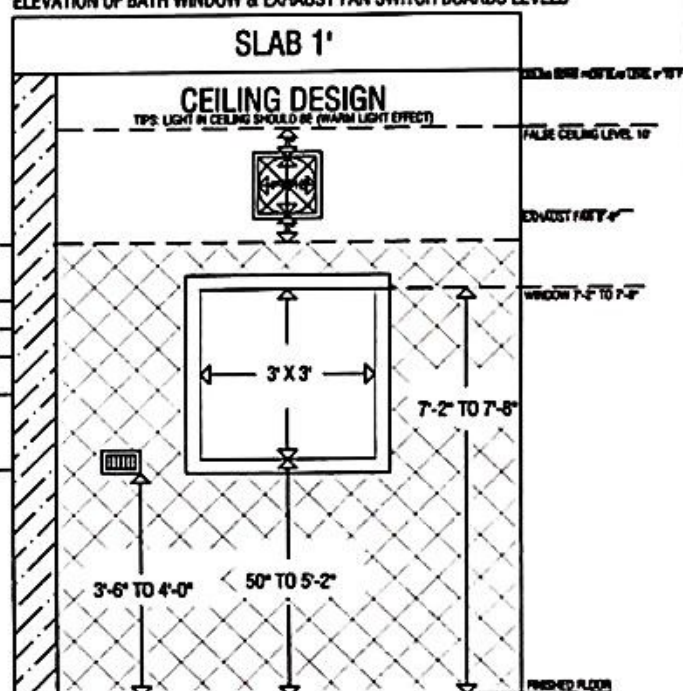
ELEVATION OF BATH WINDOW & EXHAUST FAN SWITCH BOARDS LEVELS
