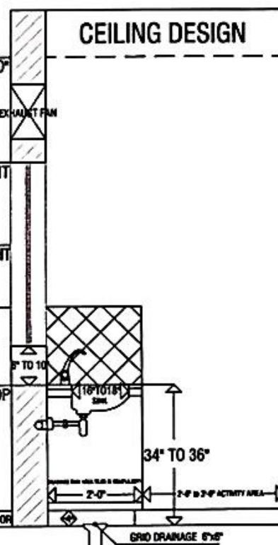
SIDE ELEVATION SINK & DRAINAGE SYSEM
