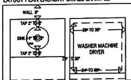
LAYOUT PLAN LAUNDRY SMALL EXAMPLE
