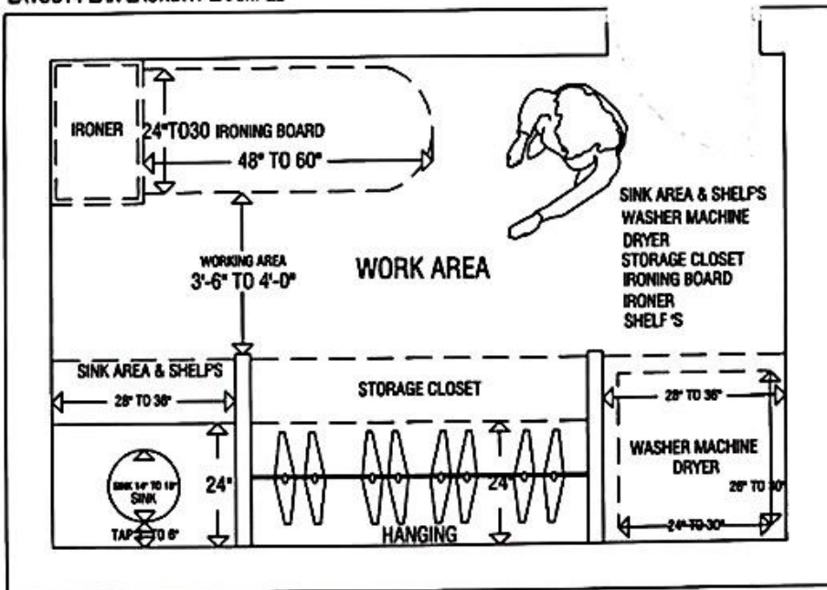
LAYOUT PLAN LAUNDRY EXAMPLE
