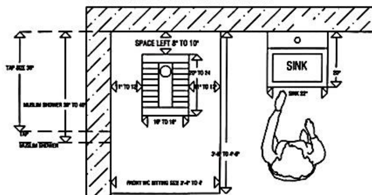
A. LAYOUT PLAN SQUAT TOILETS DETAILS
