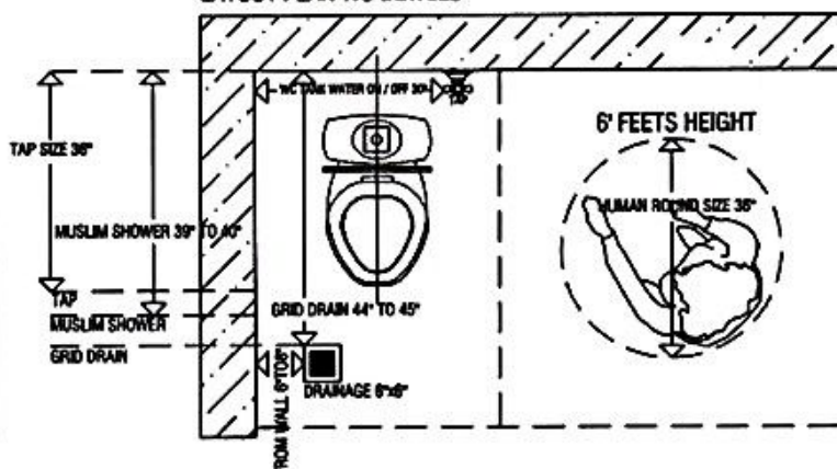
LAYOUT PLAN WC DETAILS
