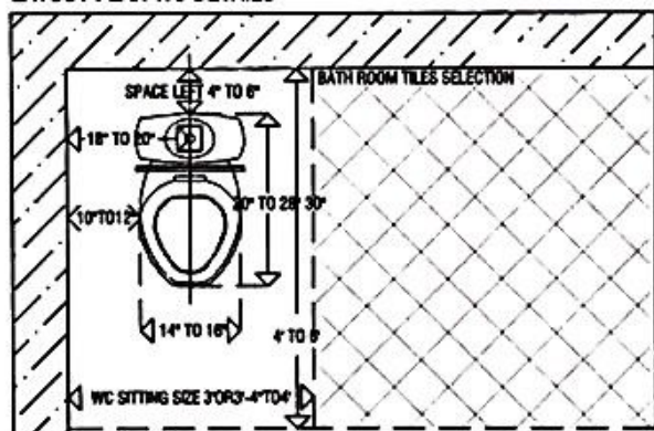
LAYOUT PLAN WC DETAILS
