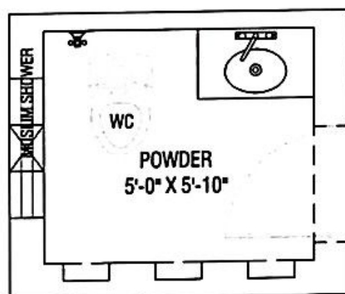
LAYOUT PLAN EXMAPLE OF SMALLEST BATH ROOM
