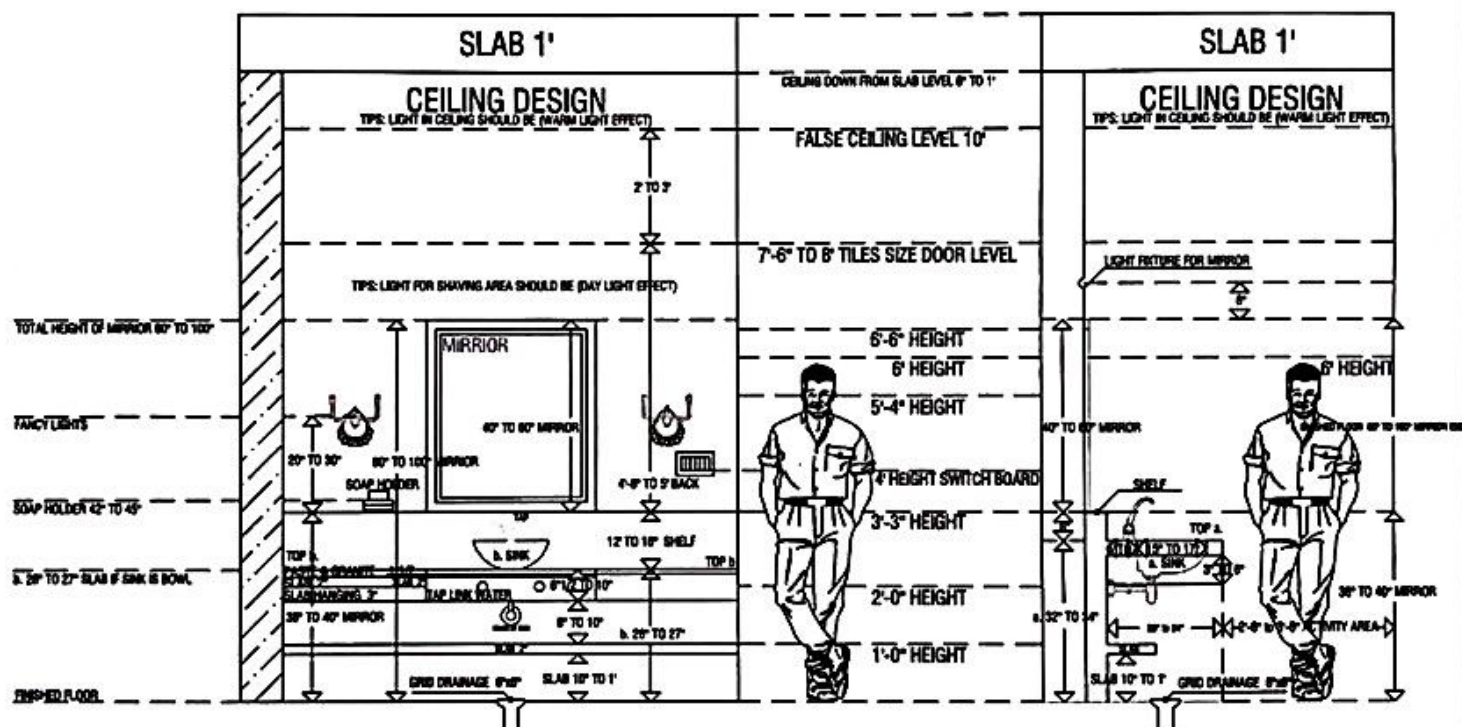
SIDE ELEVATION OF SINK & MIRROR AREA A. TYPE SINK UNDERCOUNTER
