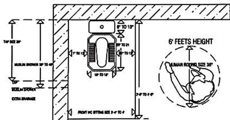
B. LAYOUT PLAN SQUAT TOILETS DETAILS
