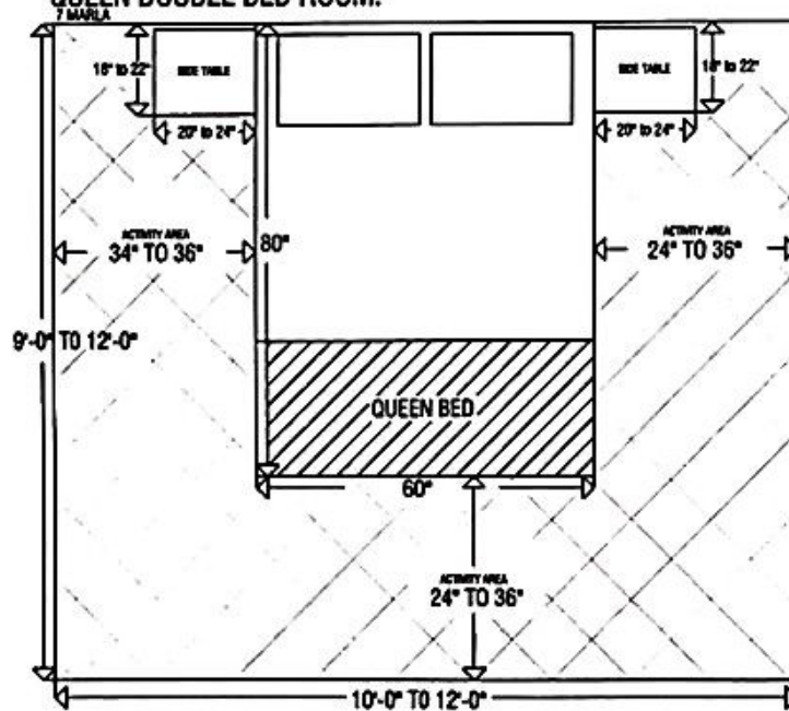
QUEEN DOUBLE BED ROOM.
