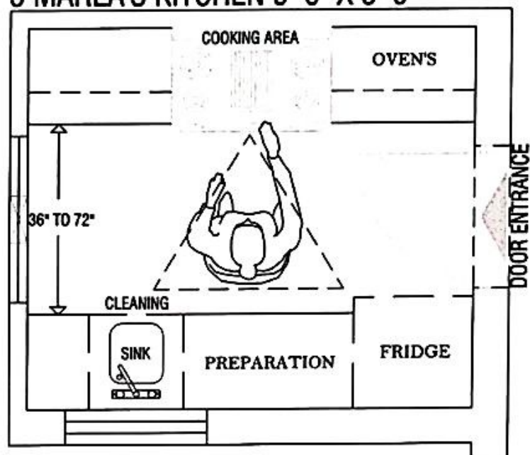
5 MARLA'S KITCHEN 9'-6" X 8'-0"
