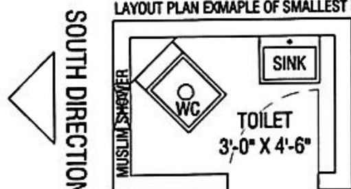
LAYOUT PLAN EXMAPLE OF SMALLEST BATH
