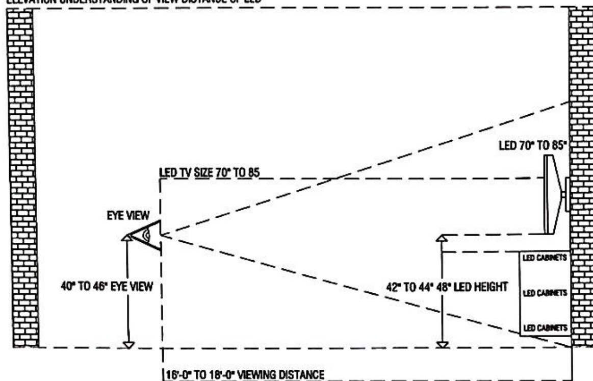
ELEVATION UNDERSTANDING OF VIEW DISTANCE OF LED
