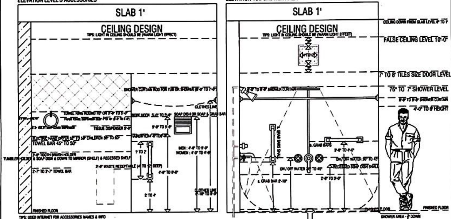
ELEVATION TUB SHOWER AREA
