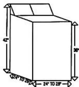
AUTOMATIC DRYER
