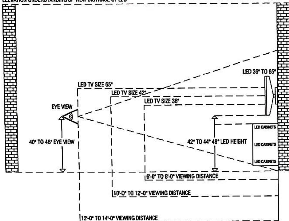
ELEVATION UNDERSTANDING OF VIEW DISTANCE OF LED
