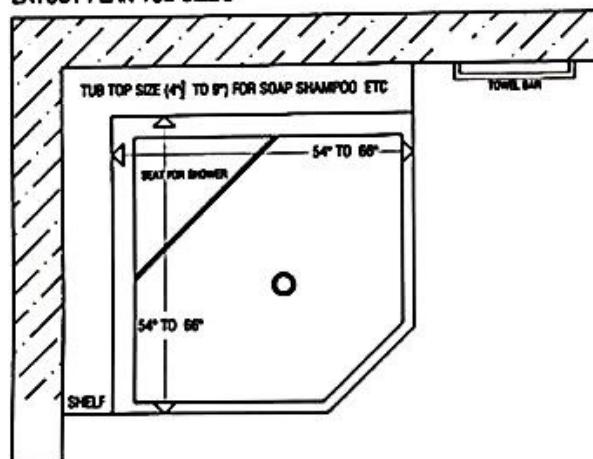
LAYOUT PLAN TUB SIZE'S
