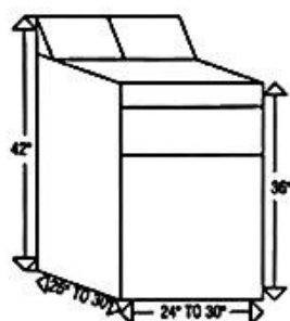
AUTOMATIC WASHER
