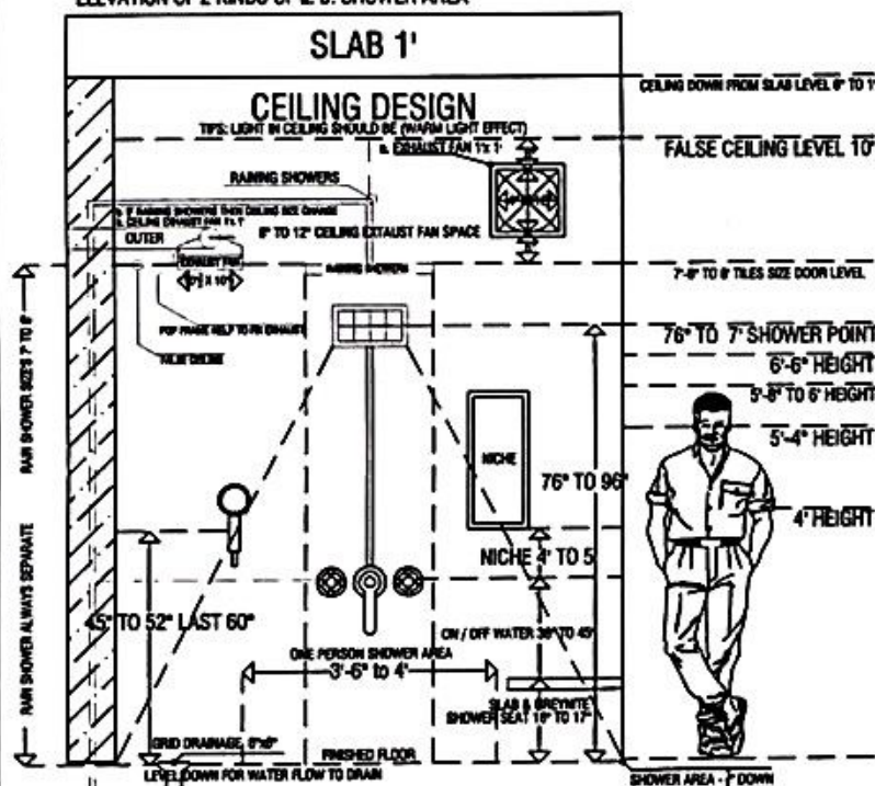
ELEVATION OF 2 KINDS OF a. b. SHOWER AREA
