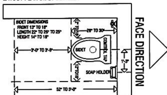
LAYOUT PLAN BIDET DETAILS
