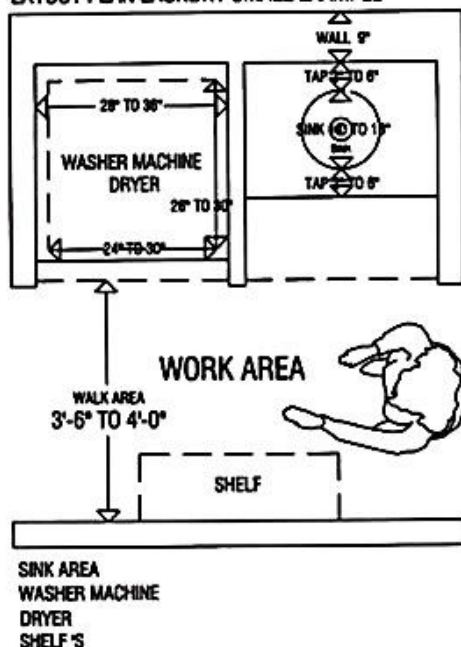
LAYOUT PLAN LAUNDRY SMALL EXAMPLE
