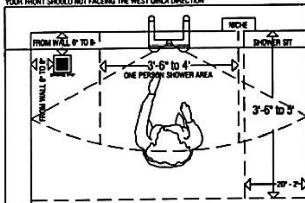
LAYOUT PLAN SHOWER DETAILS
