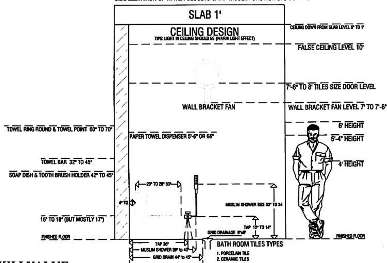
SIDE ELEVATION OF WATER CLOSETS & TAP MUSLIM SHOWER ETC DETAILS
