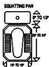
SANTARY FIXTURES STANDARD SIZE'S DETAILS
