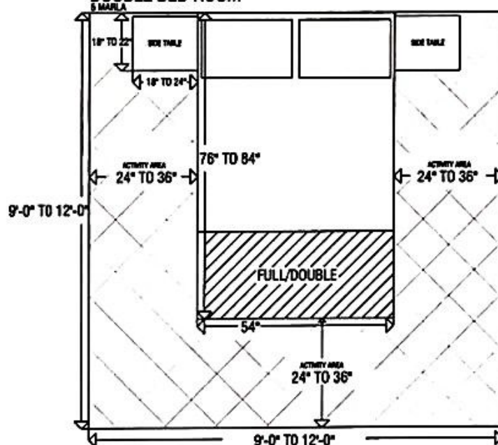
DOUBLE BED ROOM
