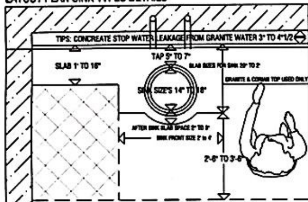
LAYOUT PLAN SINK TYPES DETAILS
